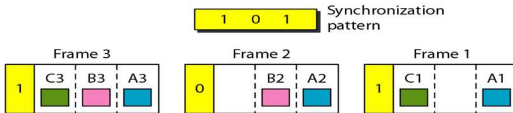
Fig24: Framing bits.
