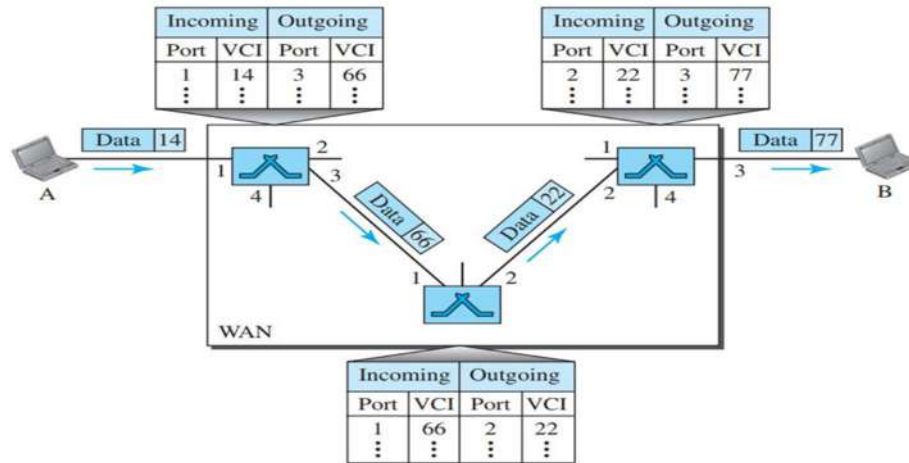
Fig: Source-to-destination data transfer in a virtual-circuit network
