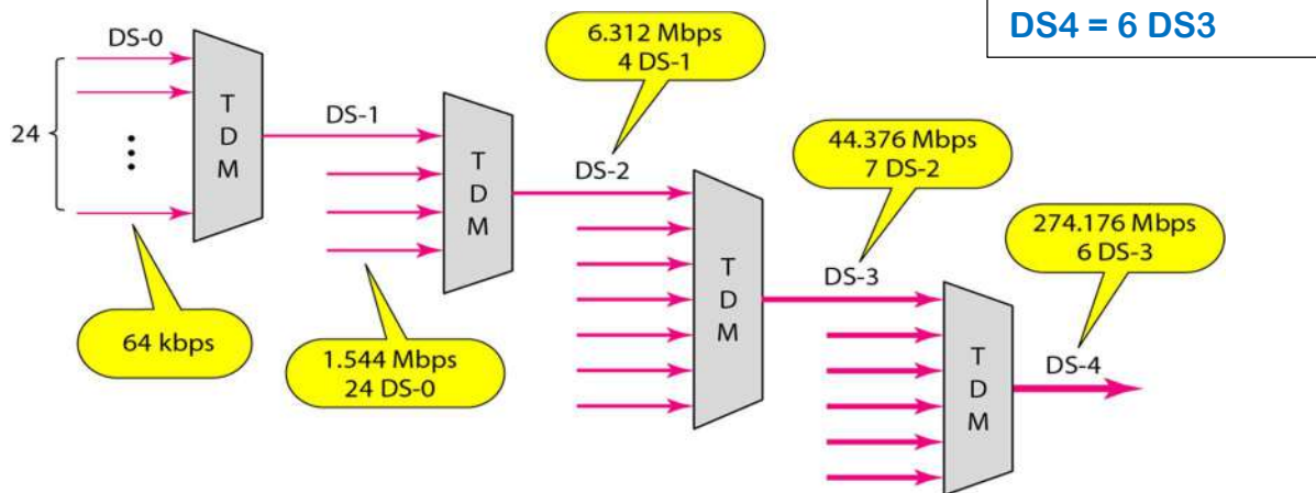
Fig25: Digital Hierarchy.
