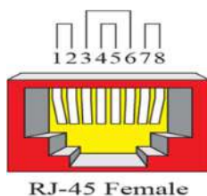
RJ-45 Female
